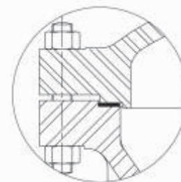
BODY-BONNET JOINT
